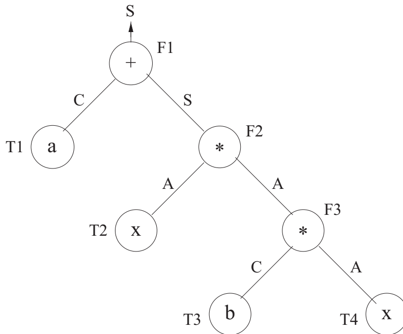
Figure 1: GP tree with symmetric output
