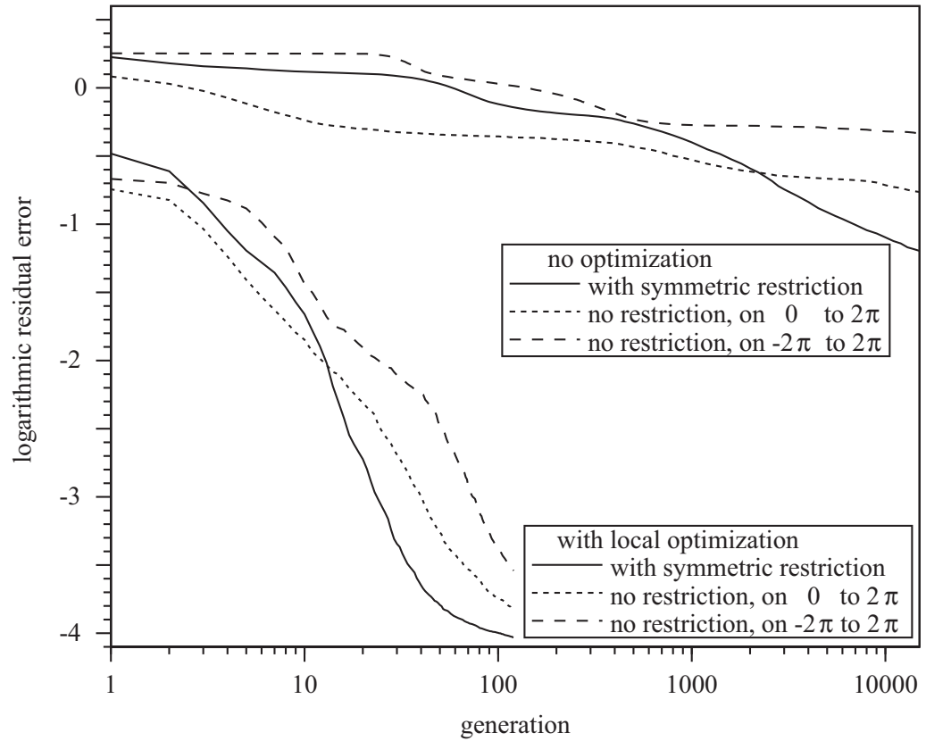
Figure 2: The mean logarithmic residual error versus the number of generations for different GP algorithms. The mean is computed over 200 GP runs, each with a population of 100 genes and an elitism rate of 50%. The runs are terminated after 120 generations with local optimization and after 15000 generations without local optimization.
