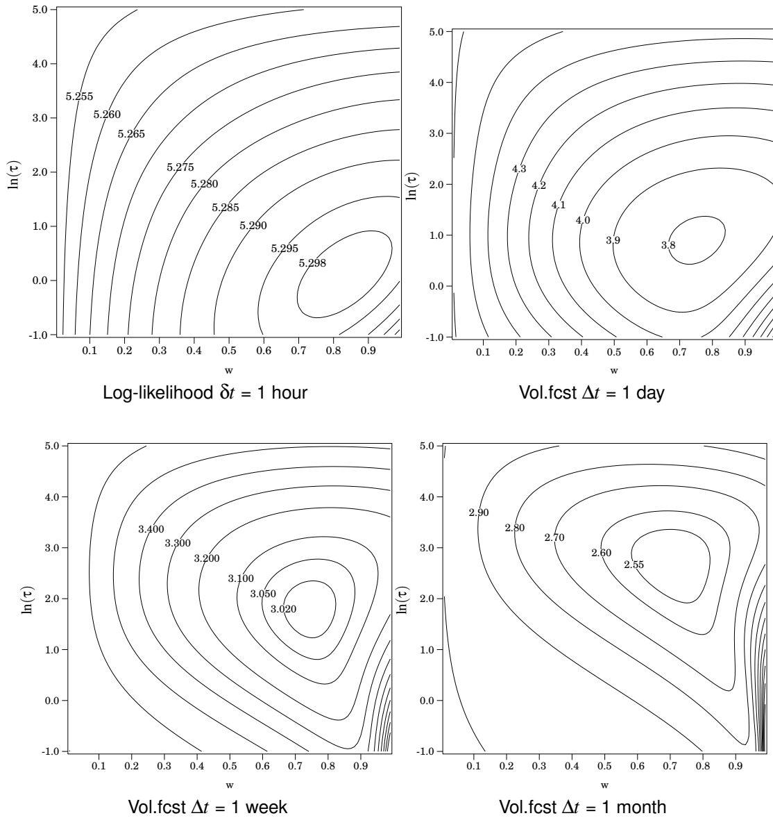
Figure 6: The cost function landscape for the GARCH(1,1) process. These figures are a cut at constant volatility \sigma in the three dimensional parameters space, with \sigma^2 = \sum r^2 the empirical volatility.
