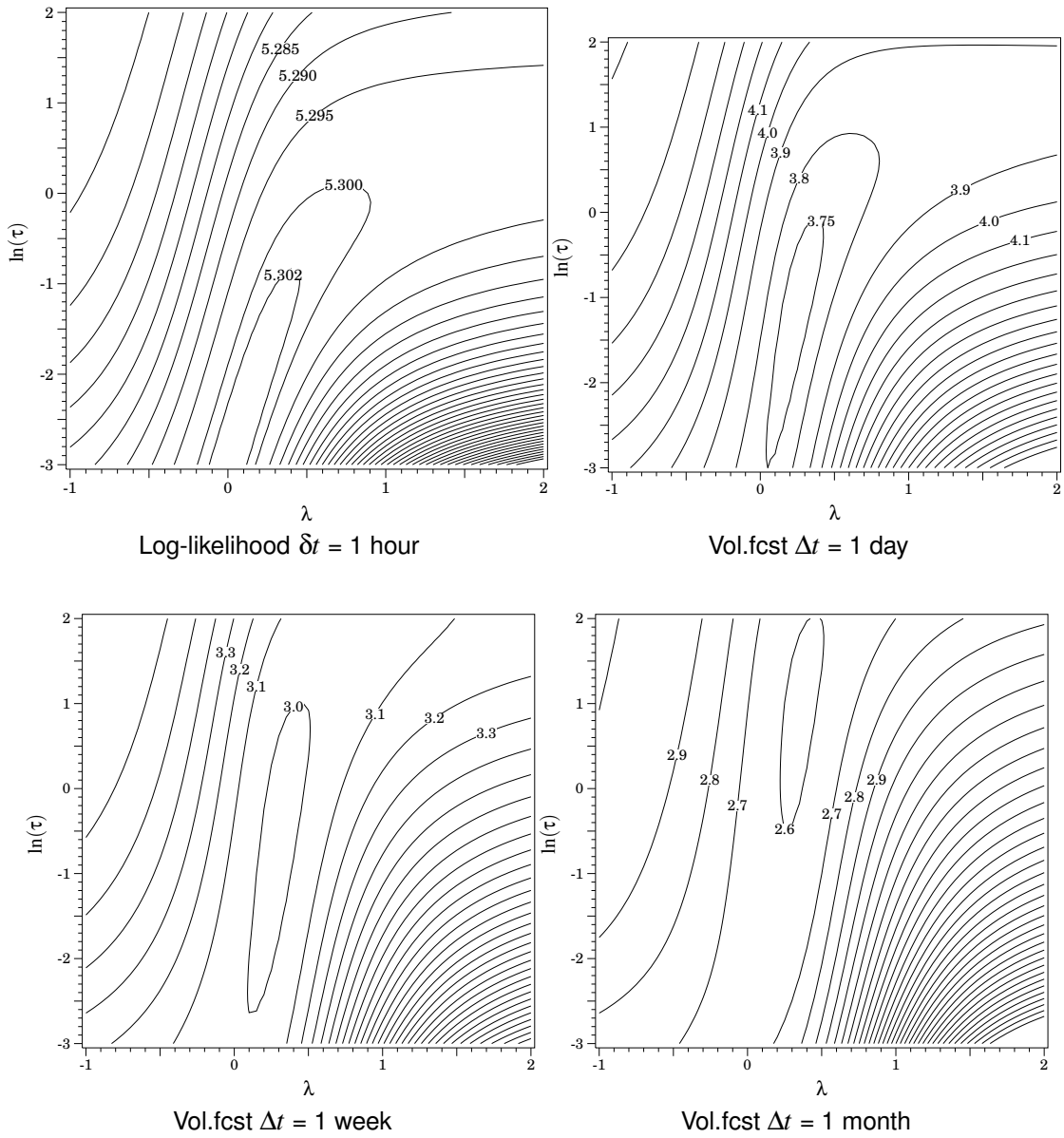
Figure 8: The cost function landscape for the LM-Mic-Lin-ARCH process.
