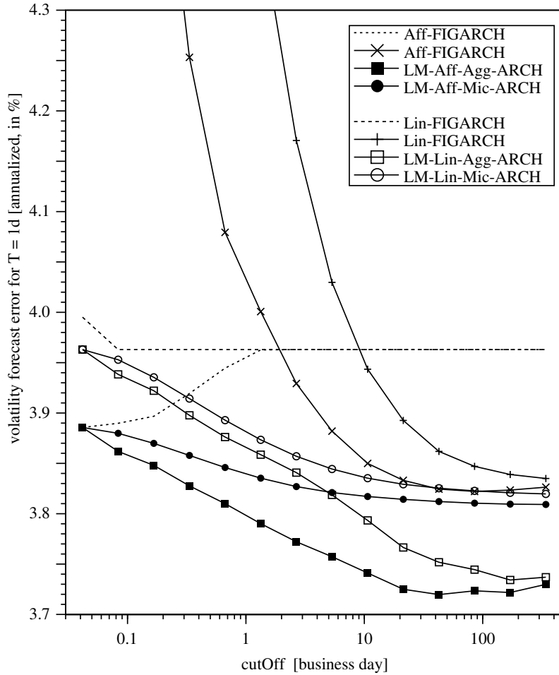
Figure 1: The one day forecast error as a function of the cut-off time.
