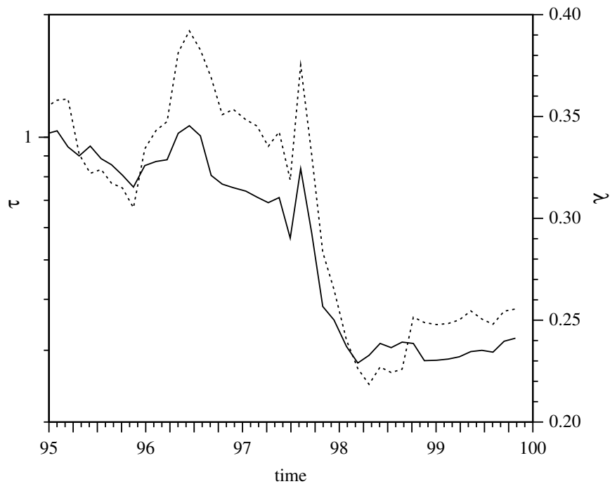
Figure 9: The parameters \tau (full line, left axis) and \lambda (dotted line, right axis) for the LM-Mic-Lin-ARCH process estimated on a moving 5 year window. The time on the horizontal axis corresponds to the end of the 5 years estimation interval.
