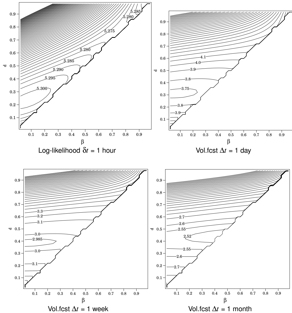
Figure 7: The cost function landscape for the Aff-FIGARCH(1,d,0) process.
