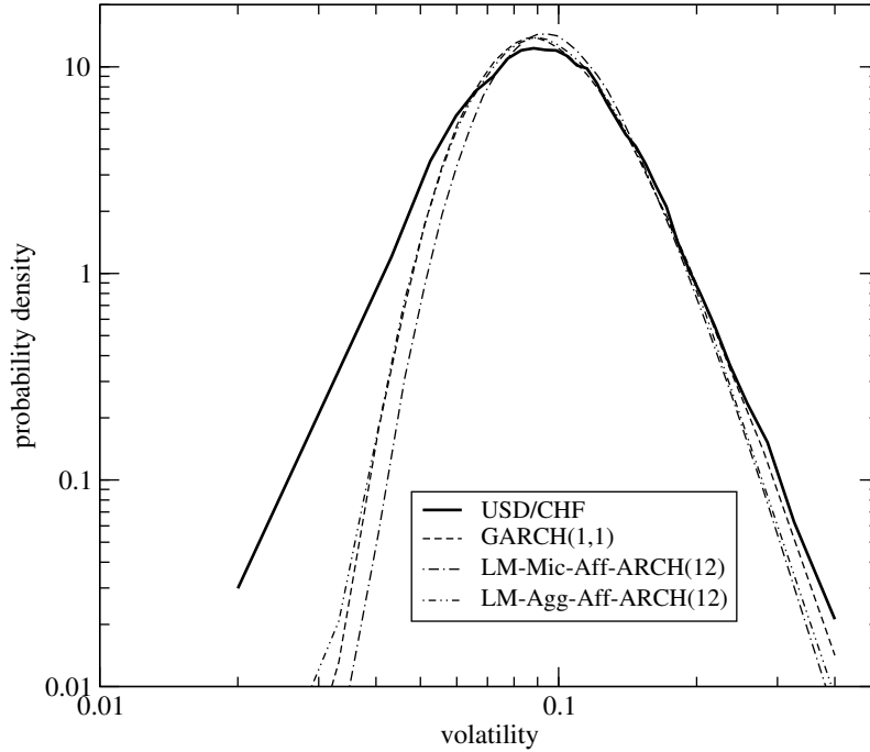
Figure 2: The volatility probability density function for some affine processes, in log-log scales. The mean volatility for all processes is the same as for the empirical data: \sigma = 11\% . The parameters are for GARCH(1,1): \alpha_1 = 0.0267 , \beta_1 = 0.966 or w_\infty = 0.218 , \tau_1 = 1.2 day; for LM-Mic-Aff-ARCH(12) and LM-Agg-Aff-ARCH(12): w_\infty = 0.123 , \tau = 0.37 day, \lambda = 0.3 . The residues \varepsilon are drawn from a Student distribution with 4.5 degrees of freedom.
